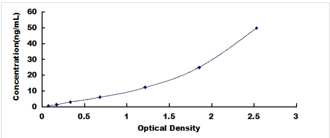
Typical Standard Curve for FTL, Rat ELISA.
