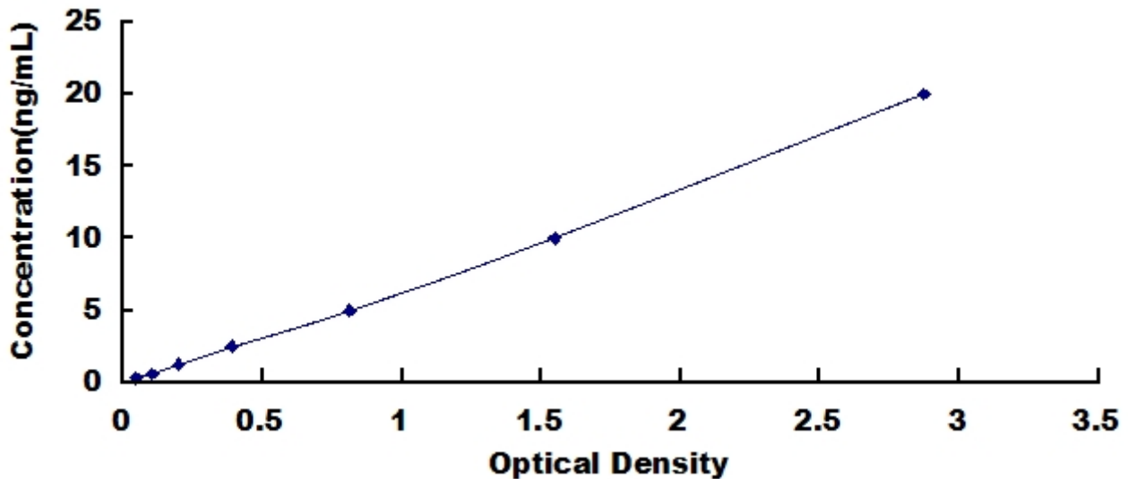
Typical Standard Curve for Ferroportin, Human ELISA.
