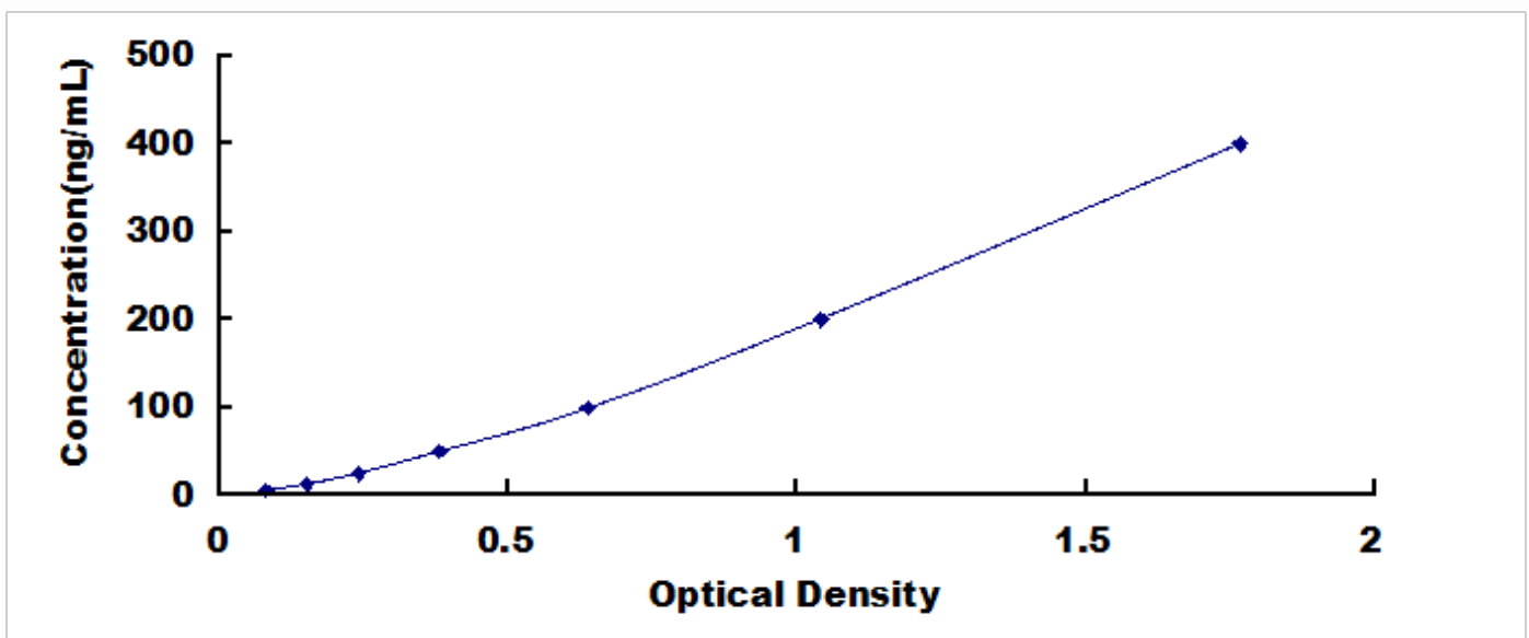
Typical Standard Curve for Fibrinogen, Mouse ELISA.
