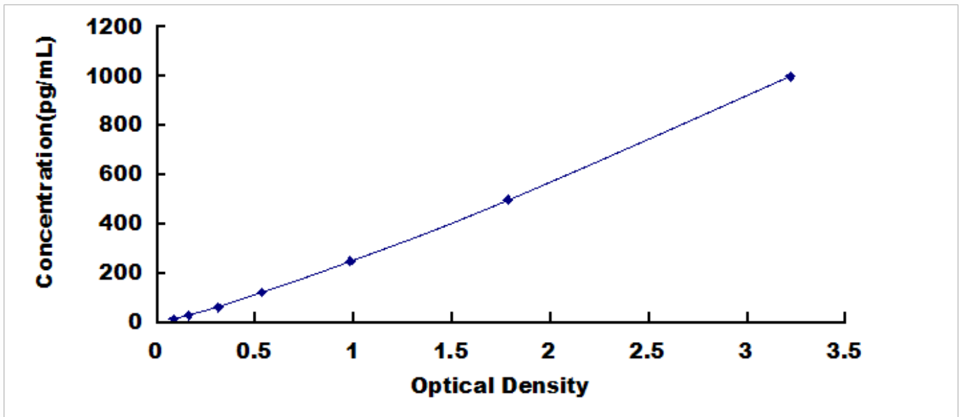
Typical Standard Curve for FGF7, Human ELISA.
