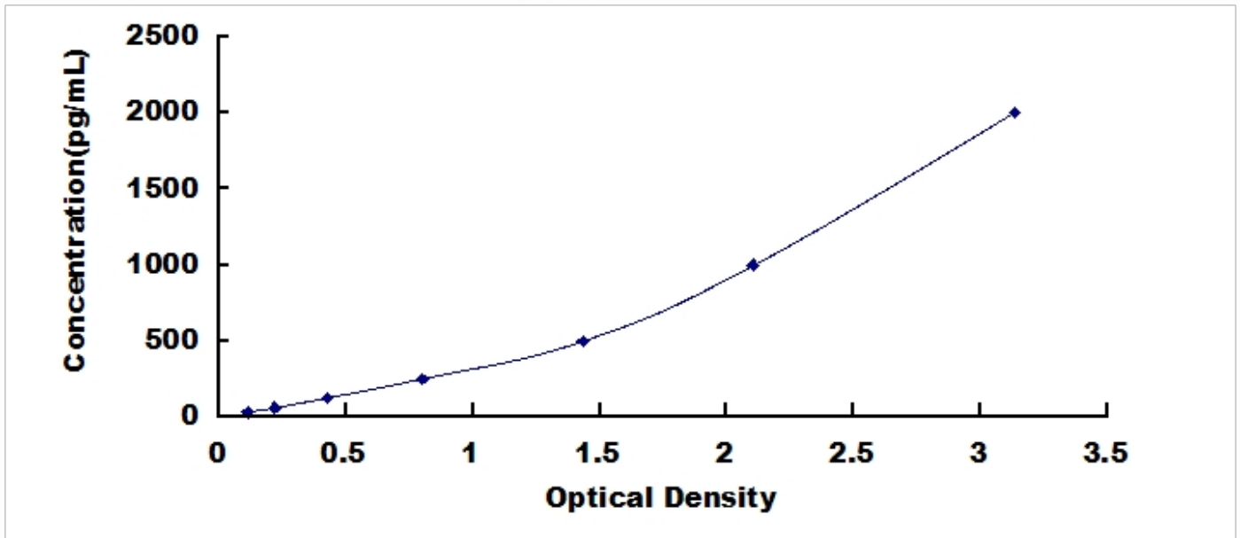
Typical Standard Curve for Fibromodulin, Human ELISA.
