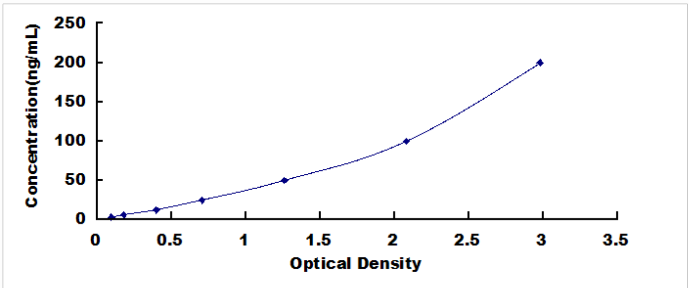
Typical Standard Curve for FBLN1, Human ELISA.
