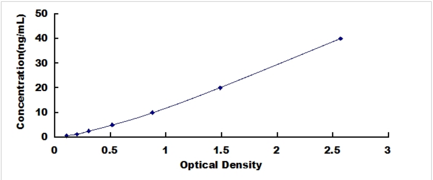
Typical Standard Curve for FCN2, Mouse ELISA.
