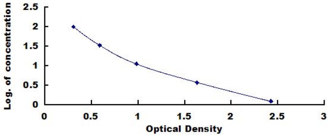
Typical Standard Curve for Follistatin, Rat ELISA.
