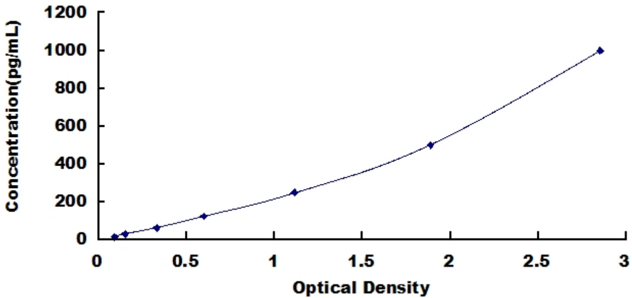
Typical Standard Curve for FUCa2, Human ELISA.
