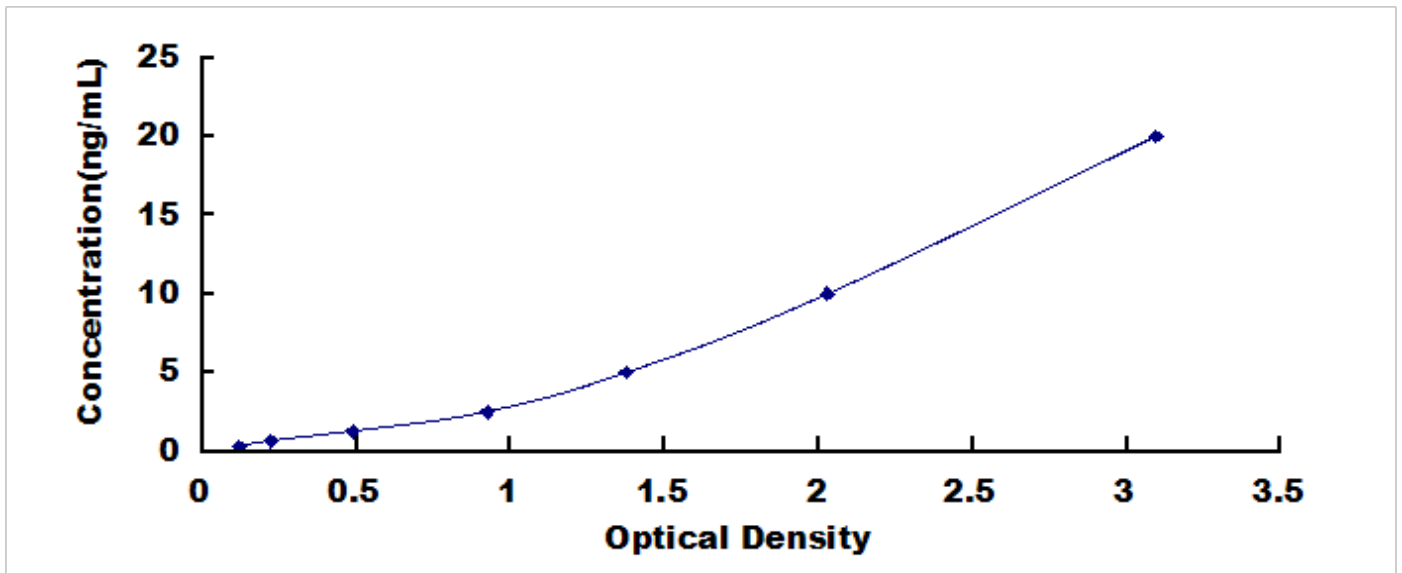
Typical Standard Curve for GPR120, Mouse ELISA.
