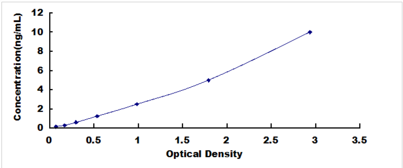
Typical Standard Curve for GAL3ST1, Human ELISA.
