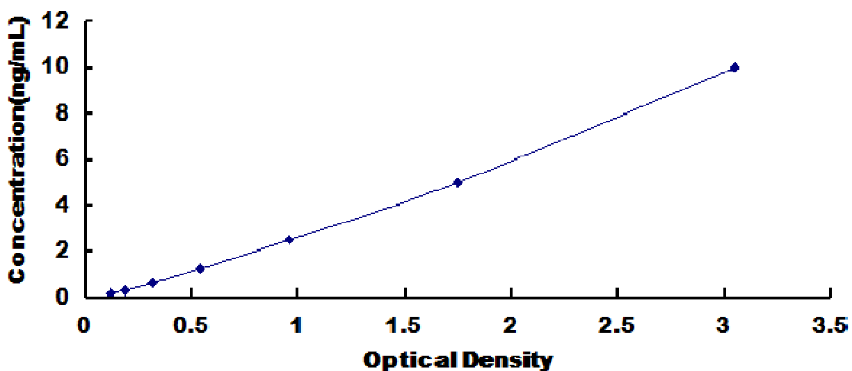
Typical Standard Curve for gABRa2, Human ELISA.
