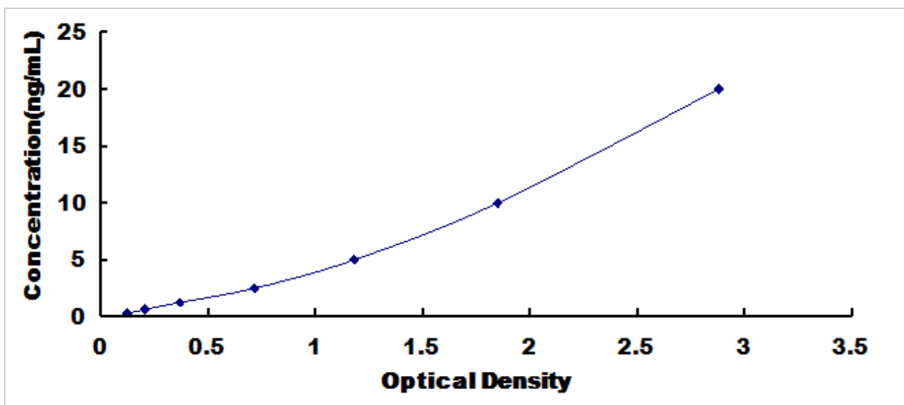
Typical Standard Curve for gSAP, Rat ELISA.
