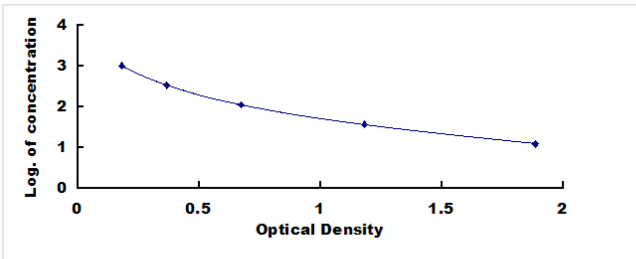
Typical Standard Curve for Ghrelin, Human ELISA.
