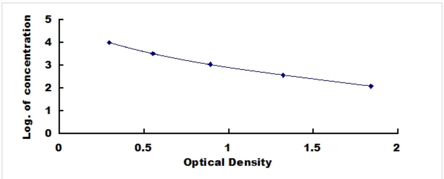
Typical Standard Curve for GLP2, Human ELISA.
