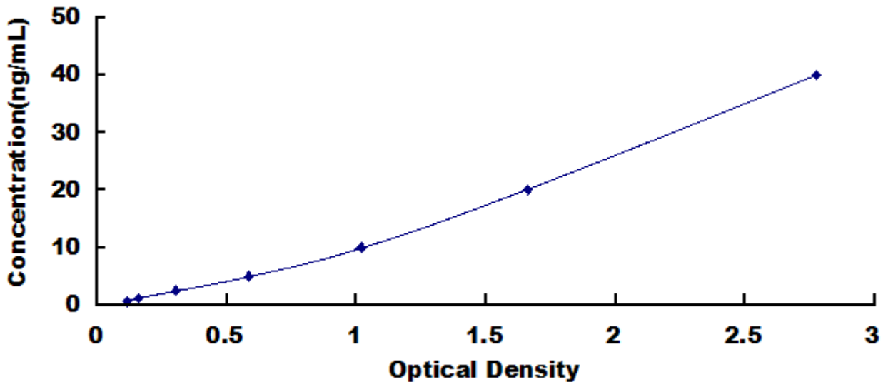
Typical Standard Curve for G6PD, Rat ELISA.
