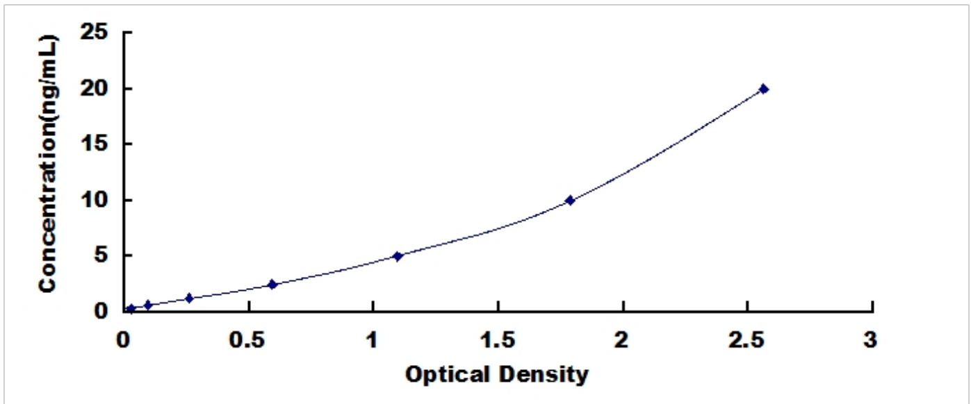
Typical Standard Curve for GLUT1, Human ELISA.
