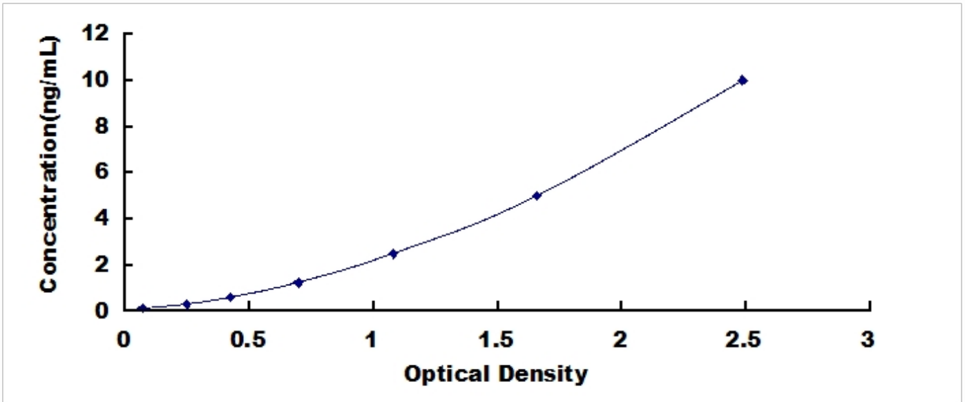
Typical Standard Curve for GDH, Human ELISA.
