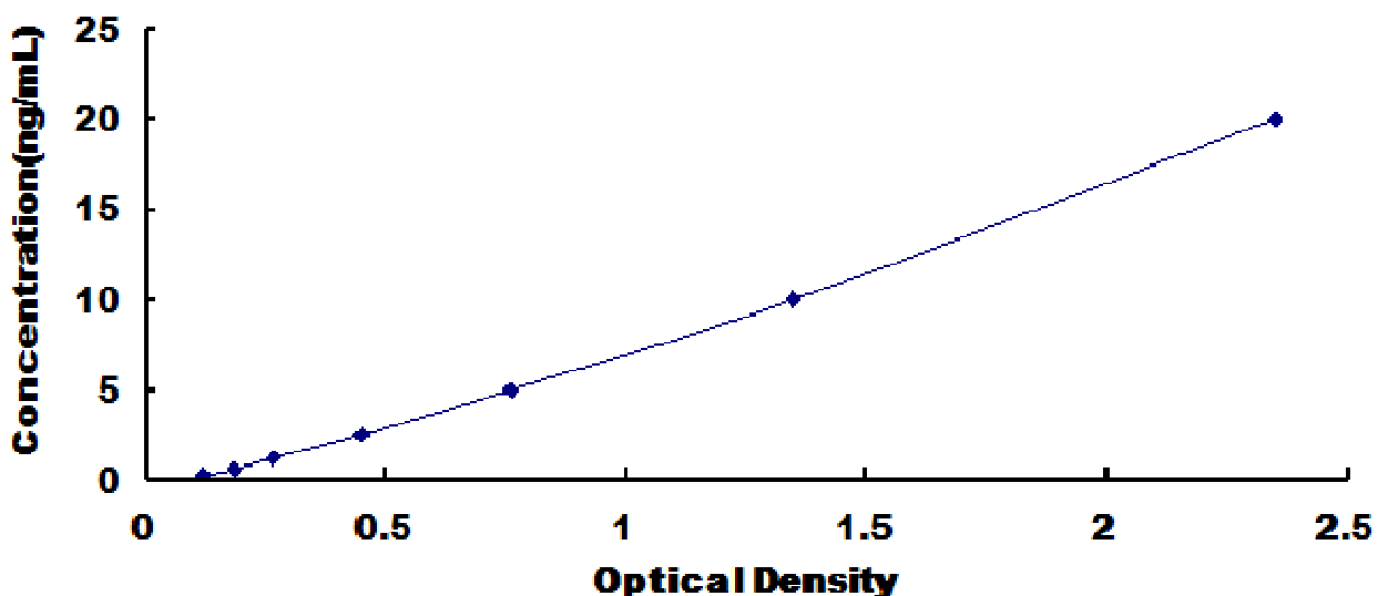
Typical Standard Curve for GRIN2D, Human ELISA.
