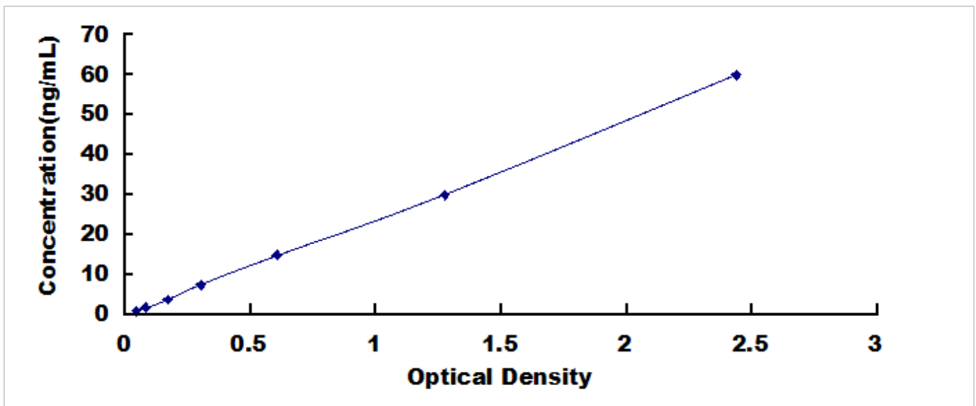
Typical Standard Curve for Glutaredoxin, Human ELISA.
