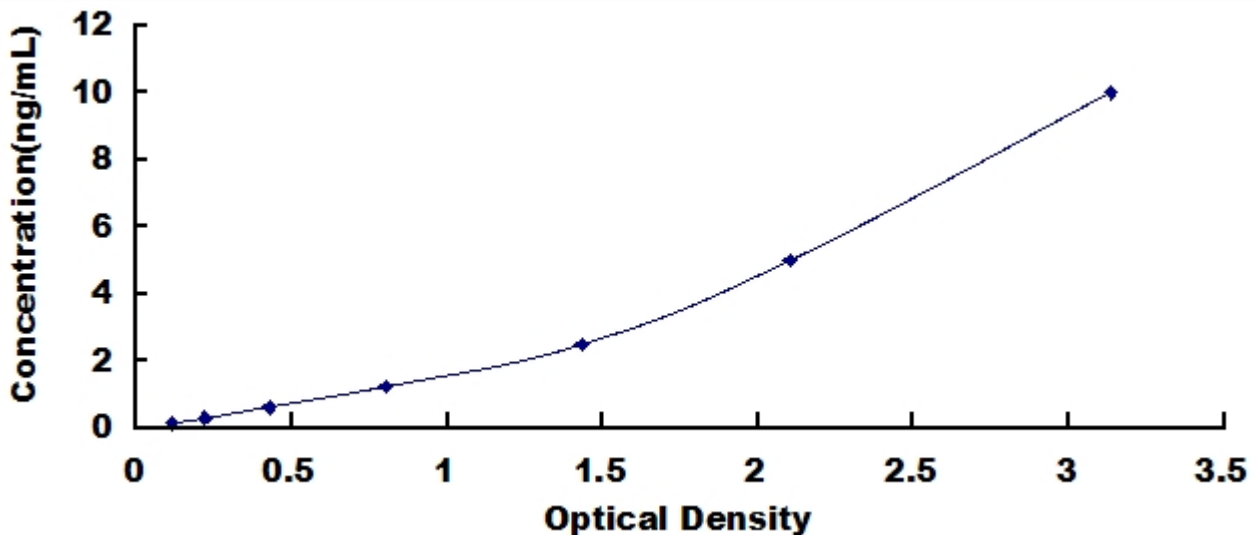
Typical Standard Curve for GPIIb/IIIa, Human ELISA.
