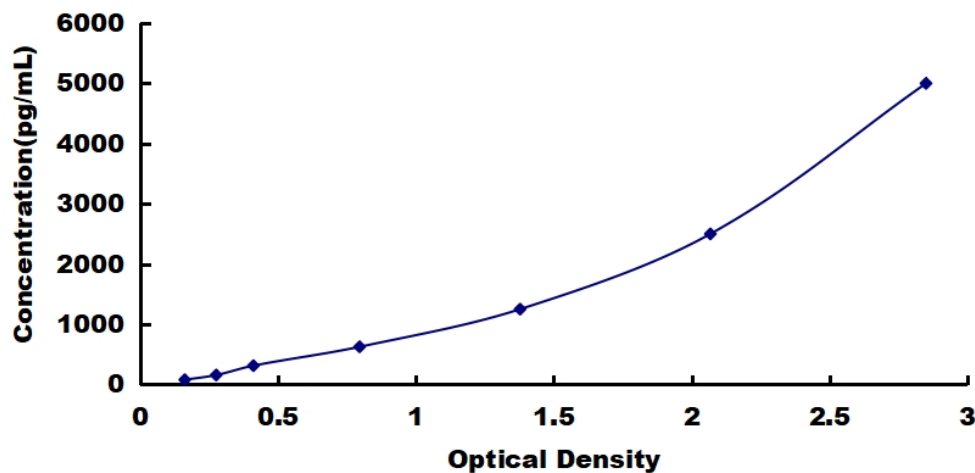
Typical Standard Curve for GLG1, Human ELISA.
