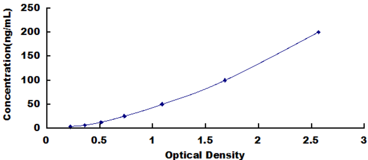
Typical Standard Curve for Haptoglobin, Canine ELISA.
