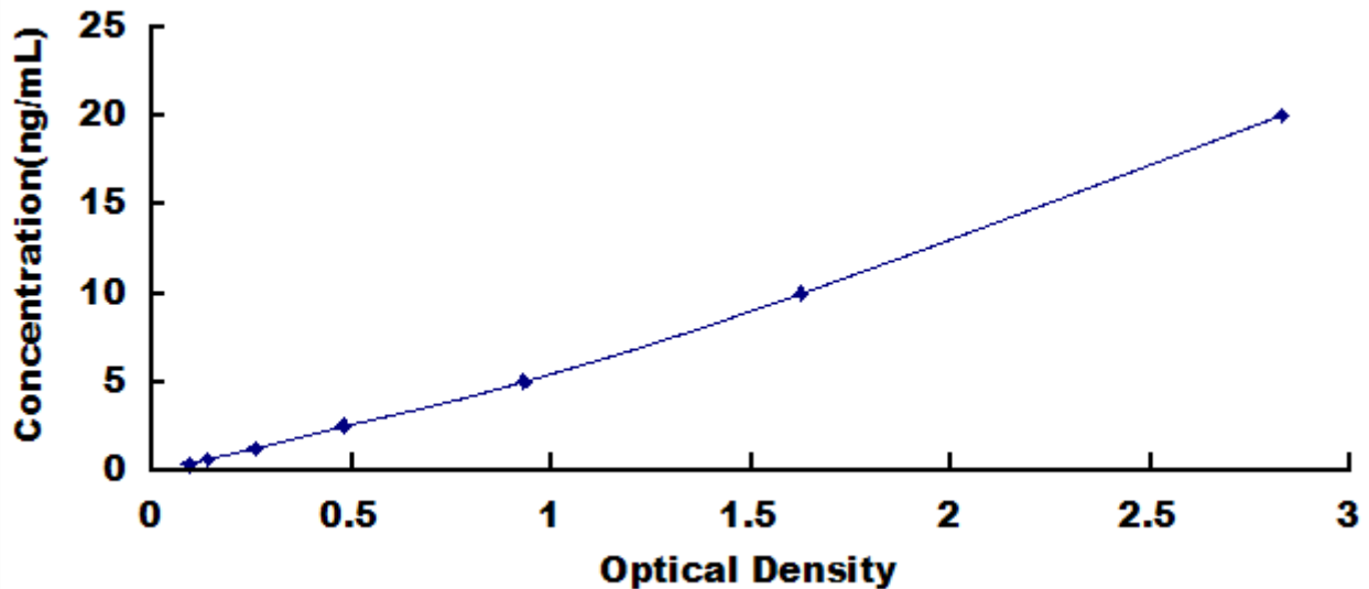
Typical Standard Curve for HSPF4, Mouse ELISA.
