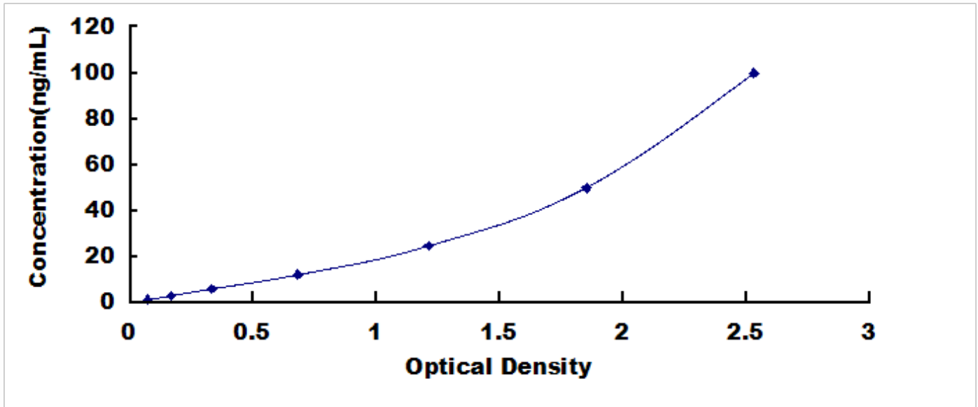
Typical Standard Curve for HSPD1, Rat ELISA.
