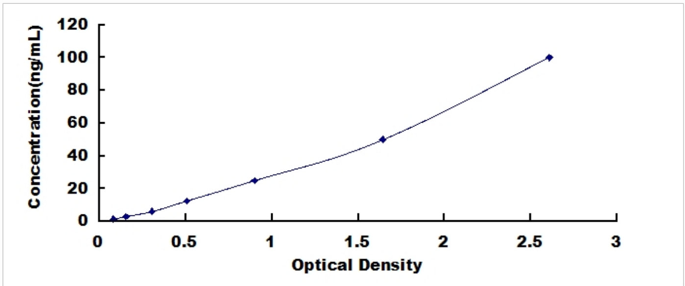
Typical Standard Curve for HbA1, Human ELISA.
