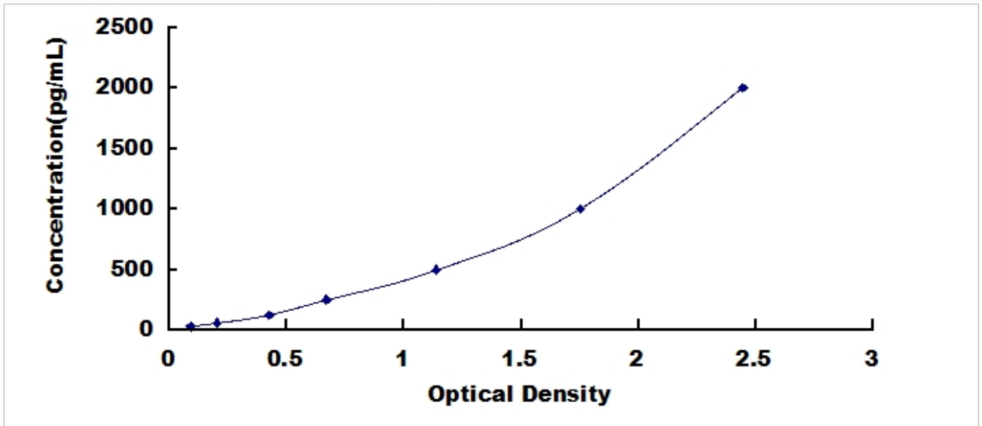
Typical Standard Curve for HMG1, Rat ELISA.
