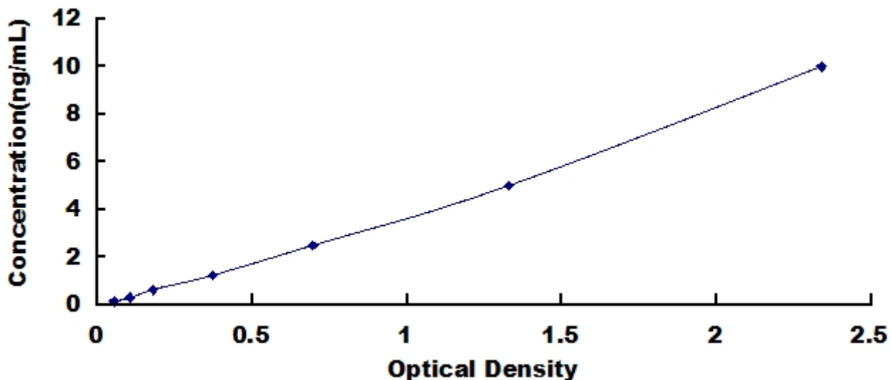
Typical Standard Curve for HOXB4, Mouse ELISA.
