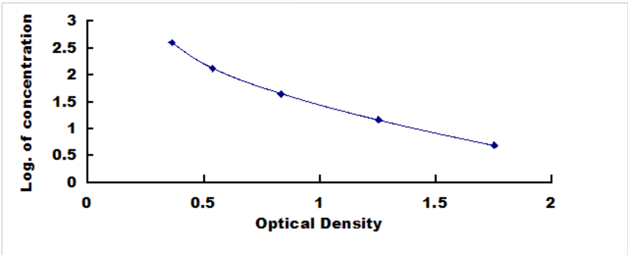
Typical Standard Curve for Hyaluronic Acid ELISA.
