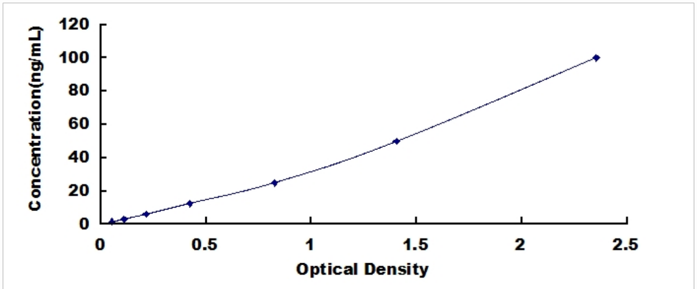
Typical Standard Curve for HAGH, Mouse ELISA.
