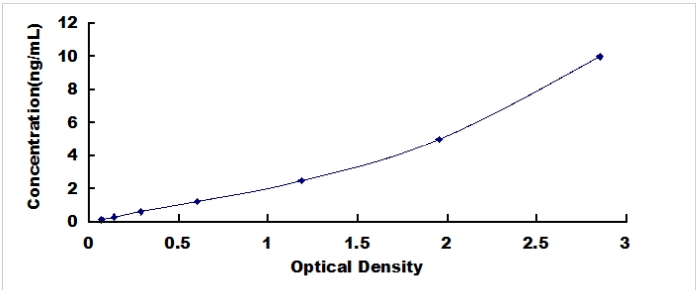
Typical Standard Curve for HIF1a, Rabbit ELISA.
