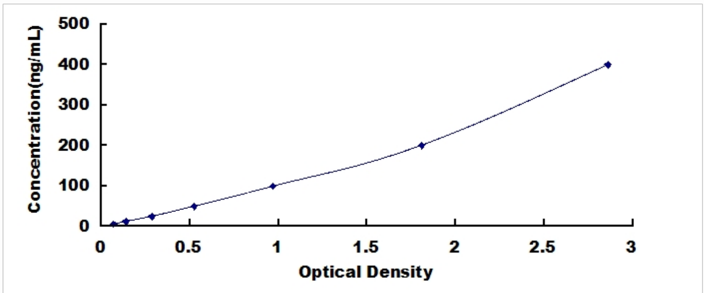
Typical Standard Curve for IgG1, Human ELISA.
