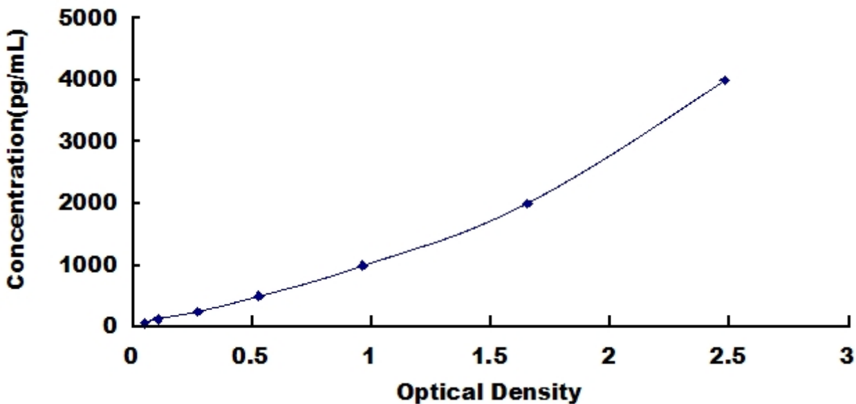
Typical Standard Curve for IgG2b, Mouse ELISA.
