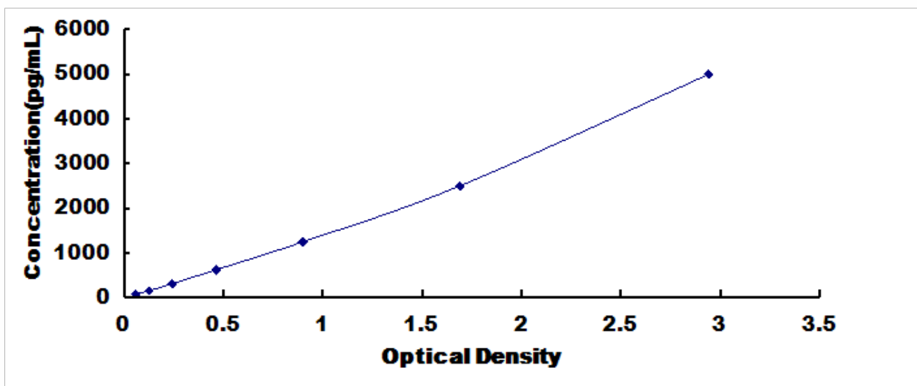
Typical Standard Curve for INHbC, Rat ELISA.
