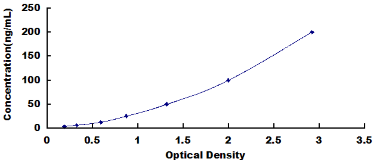
Typical Standard Curve for IGF2, Bovine ELISA.
