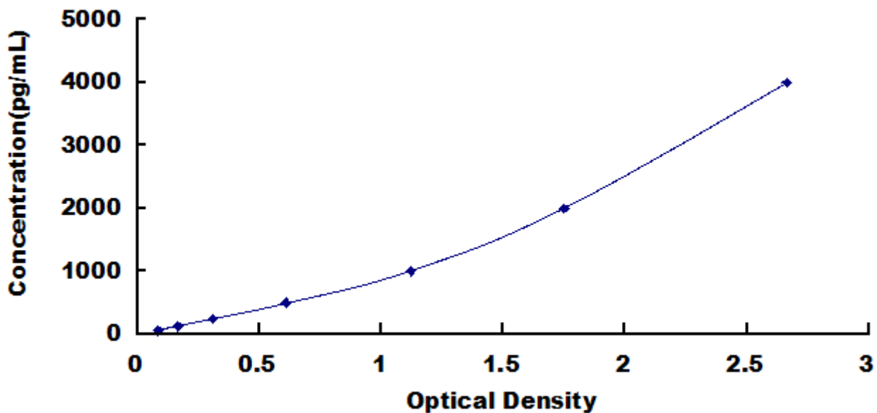
Typical Standard Curve for IGFBP2, Rat ELISA.
