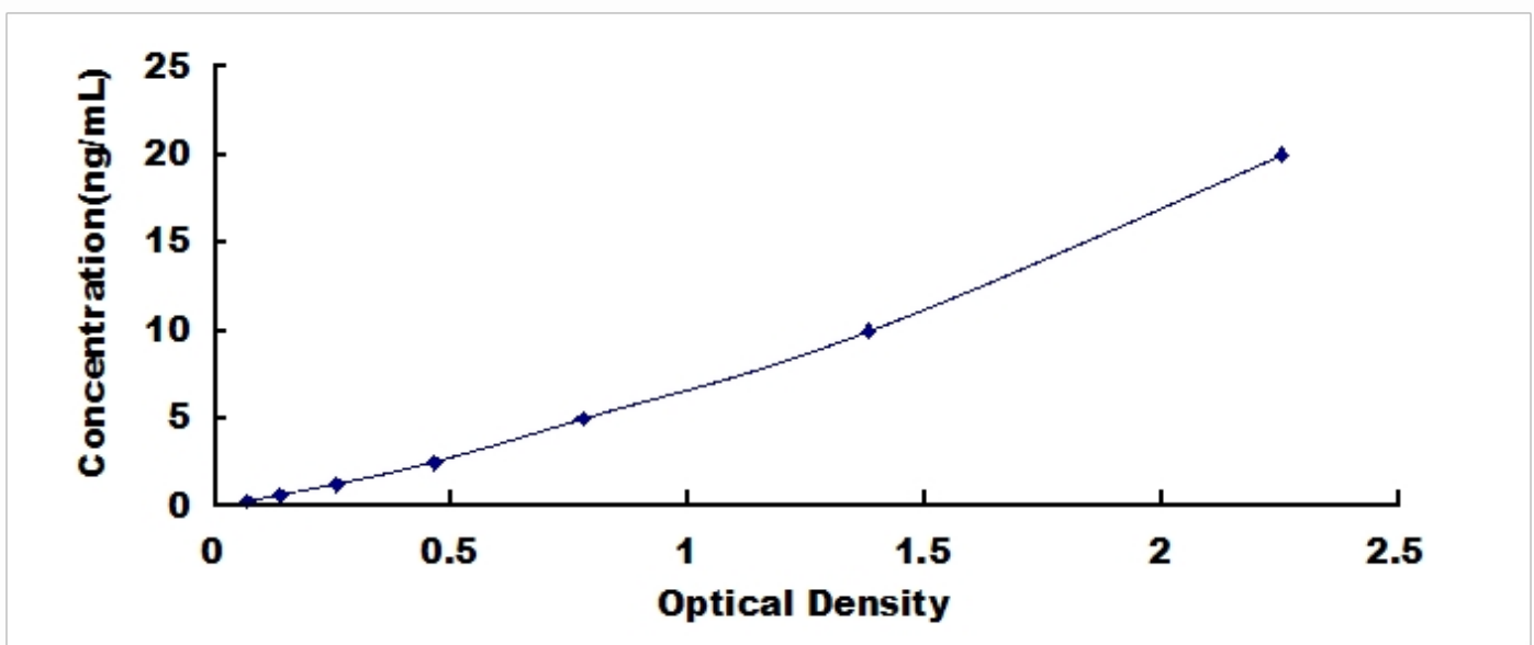
Typical Standard Curve for IGFBP4, Human ELISA.
