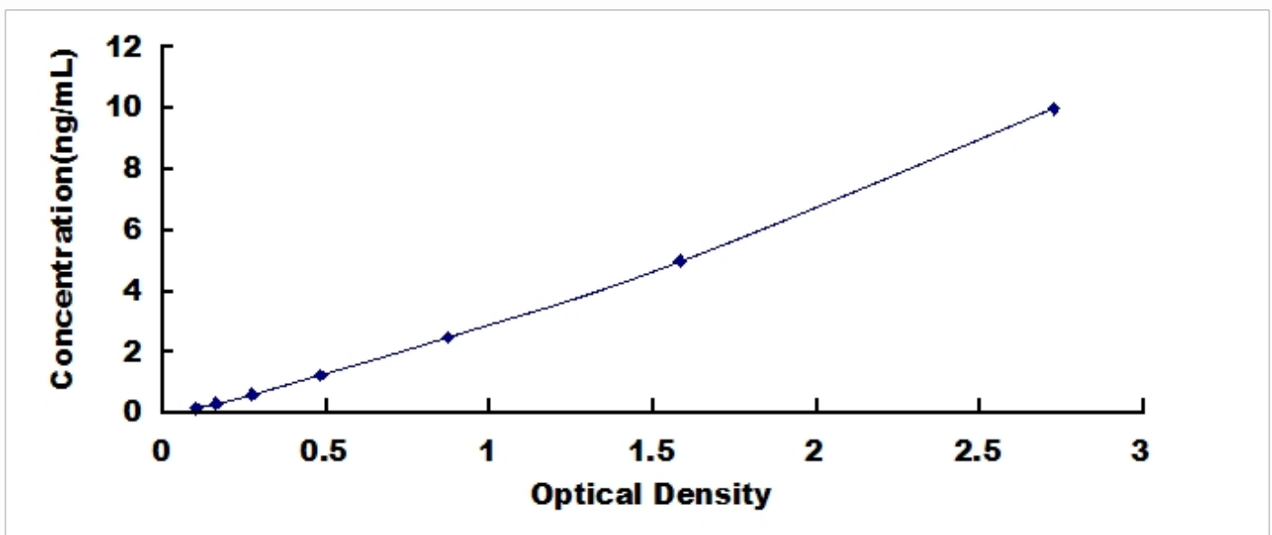
Typical Standard Curve for IGFBP5, Human ELISA.
