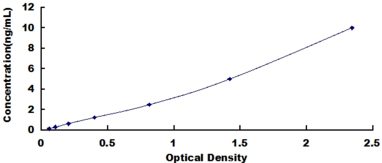
Typical Standard Curve for ITGa6, Human ELISA.
