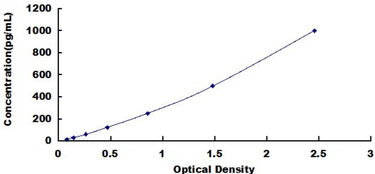
Typical Standard Curve for IFNa4, Human ELISA.
