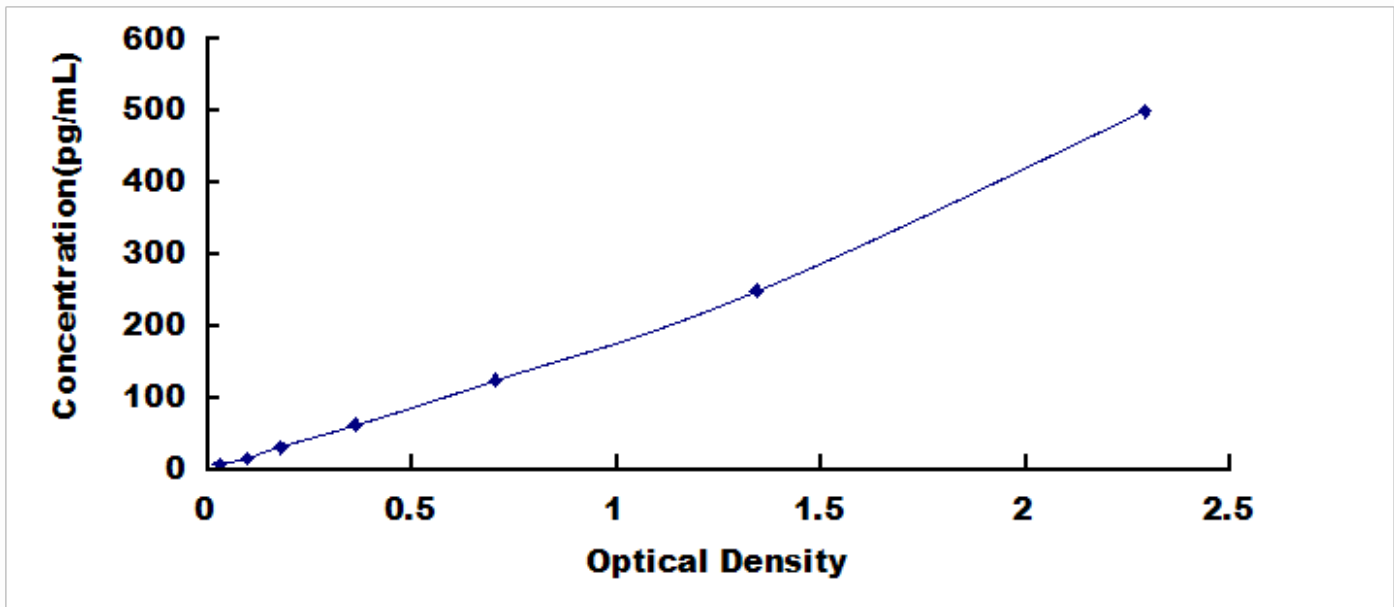
Typical Standard Curve for IL1b, Rabbit ELISA.
