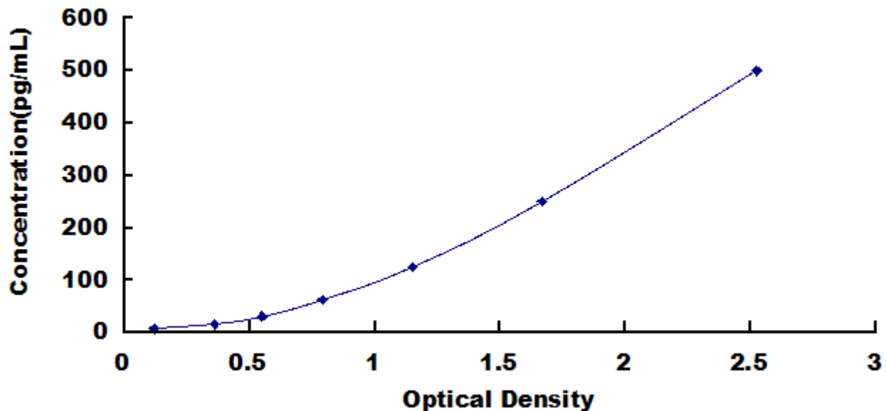
Typical Standard Curve for IL10, Rabbit ELISA.
