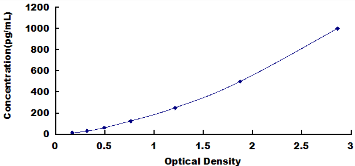
Typical Standard Curve for IL5, Gallus ELISA.
