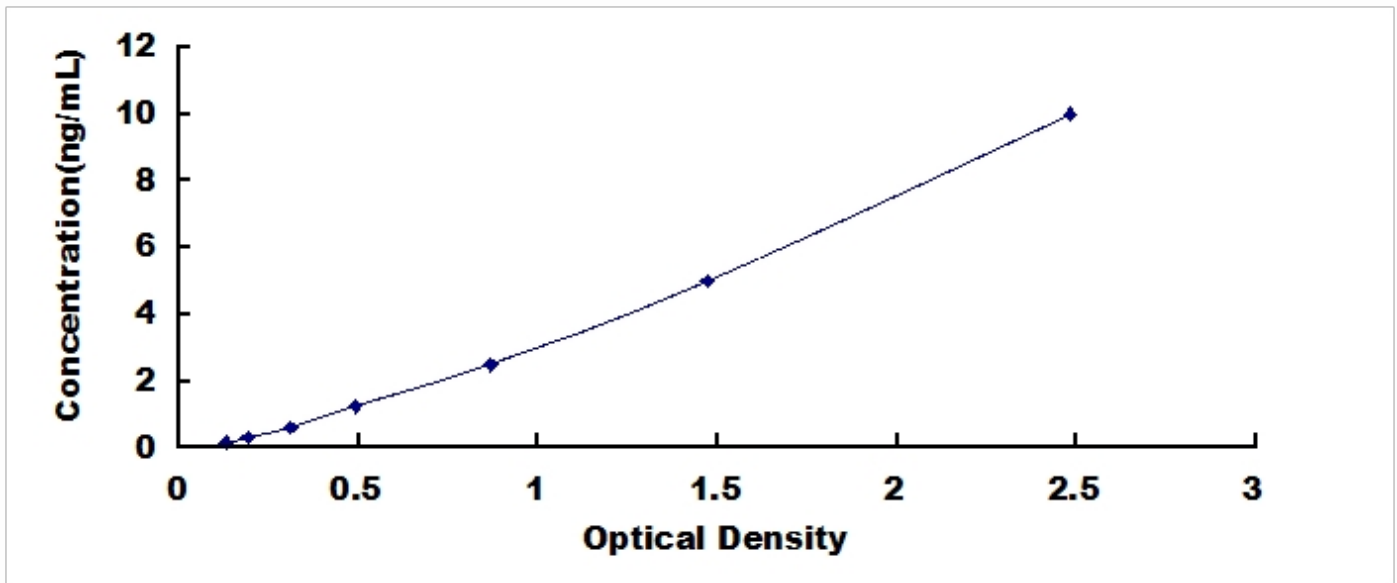
Typical Standard Curve for KLK9, Human ELISA.
