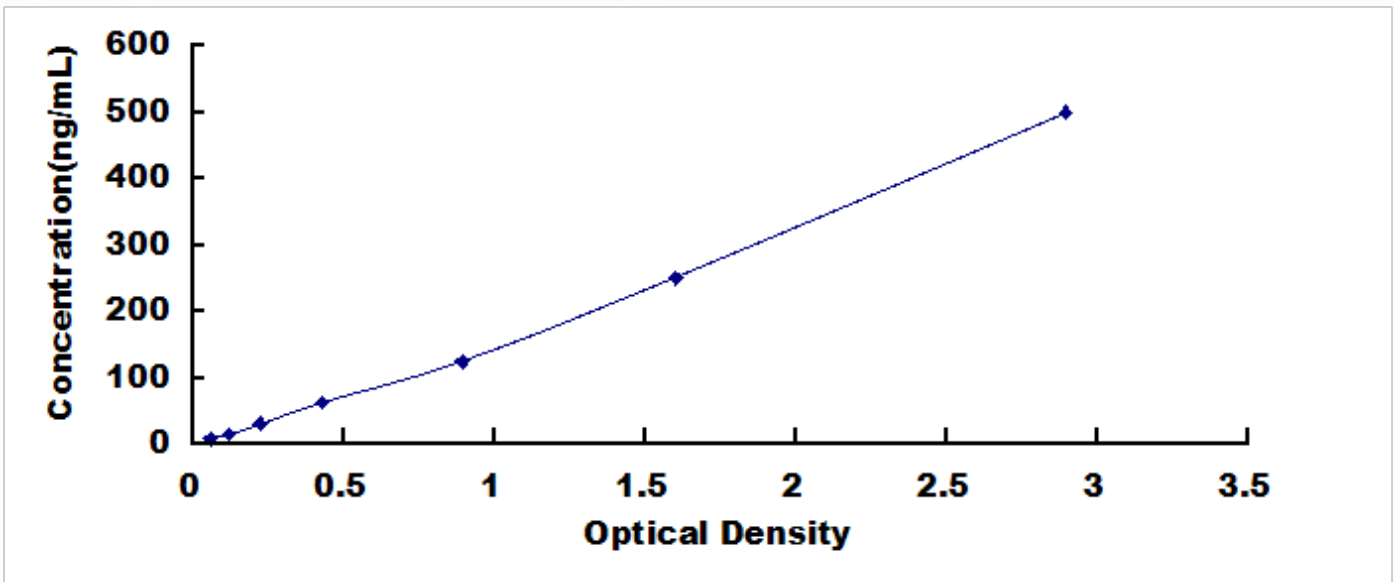
Typical Standard Curve for LDH, Mouse ELISA.
