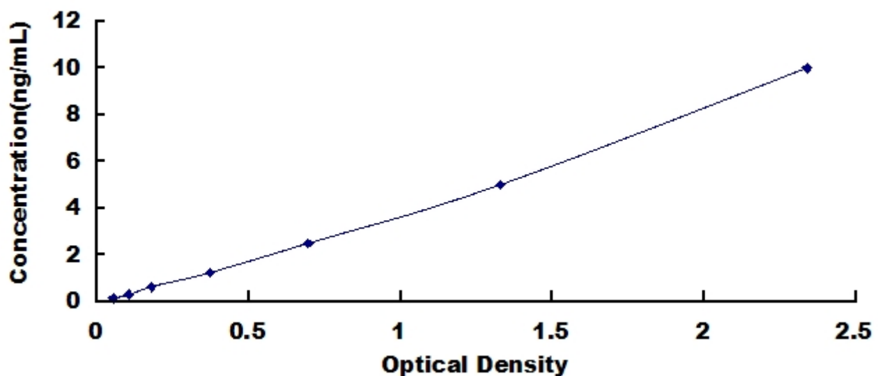
Typical Standard Curve for Lactoperoxidase, Mouse ELISA.
