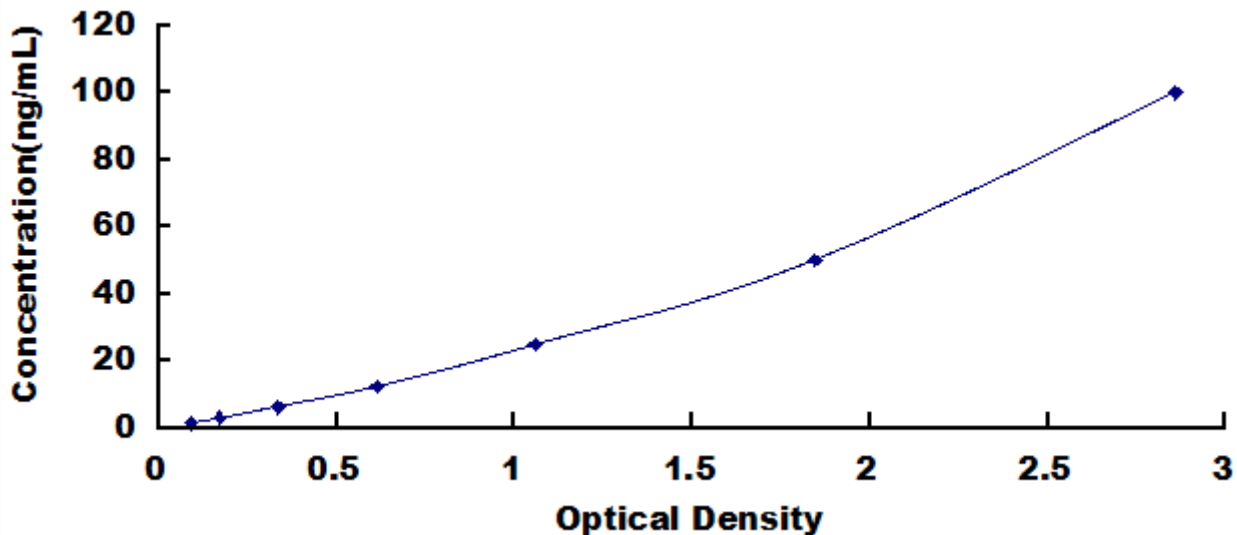
Typical Standard Curve for LGALS3BP, Rat ELISA.
