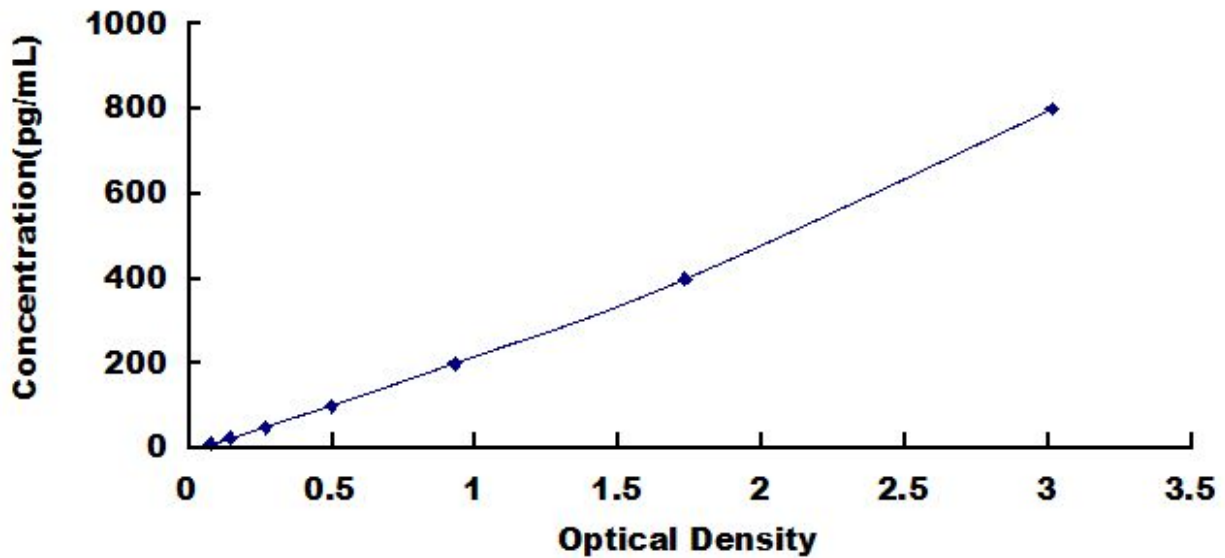
Typical Standard Curve for LOX1, Mouse ELISA.
