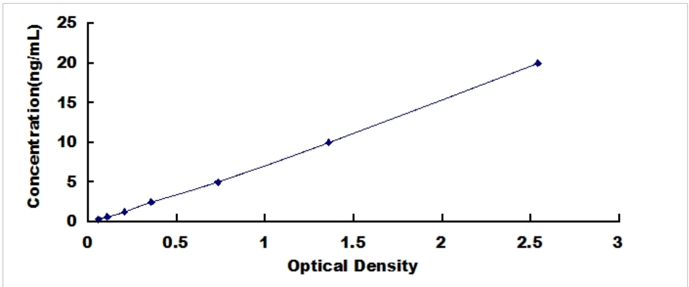
Typical Standard Curve for LRRFIP1, Human ELISA.
