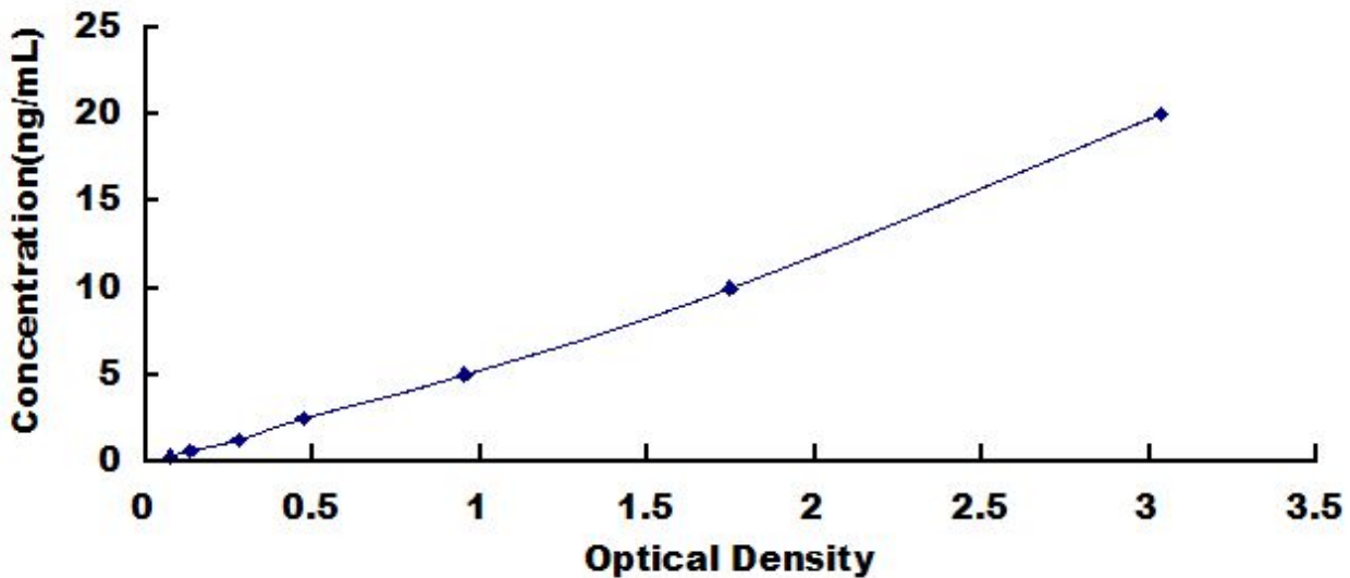
Typical Standard Curve for LRP3, Human ELISA.
